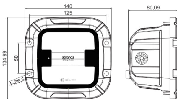
(WITH FLUSH MOUNT FRAME)
