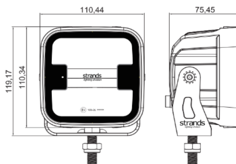
(WITHOUT FLUSH MOUNT FRAME)
